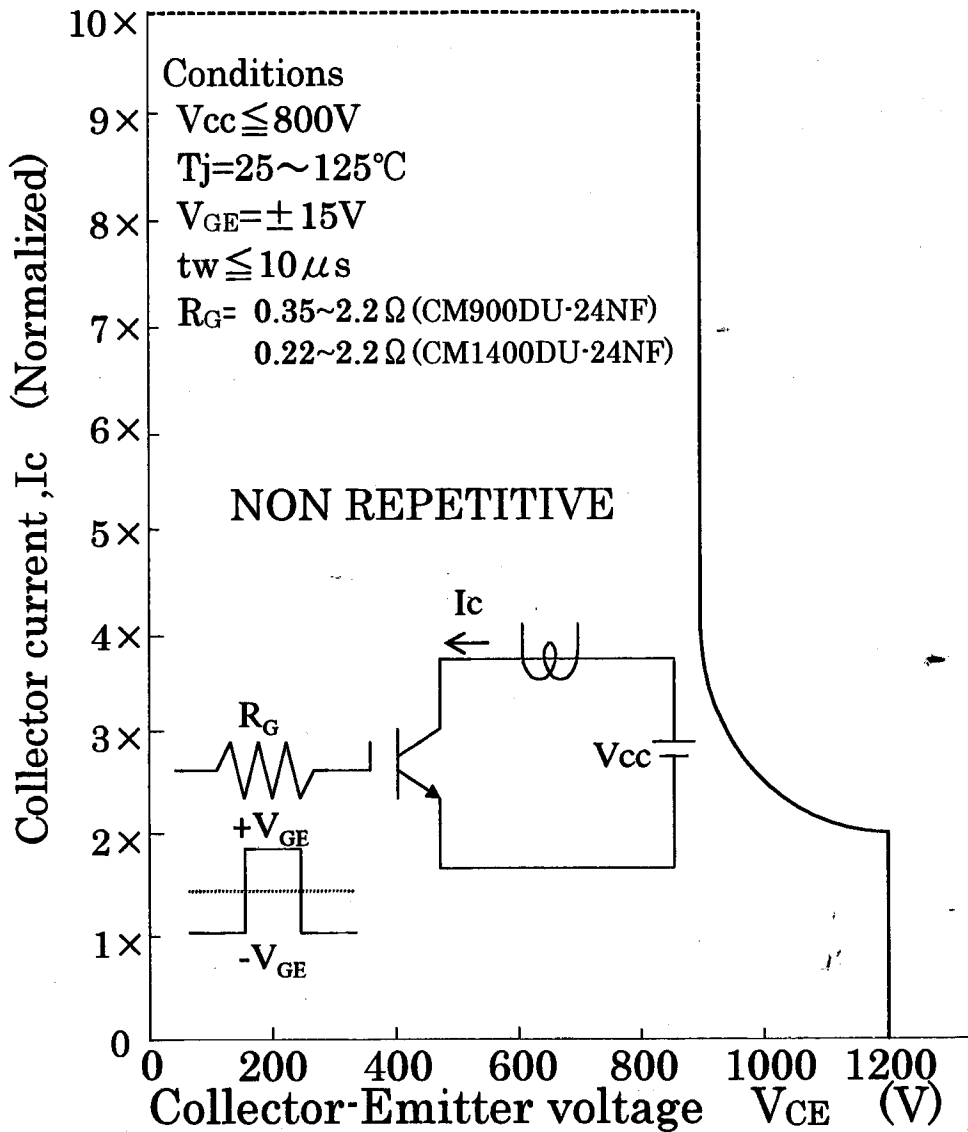
SC-SOA curve
